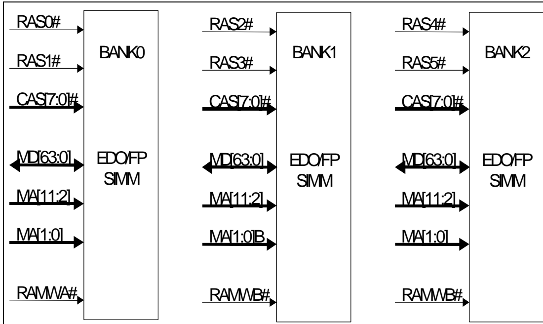
Figure 5.2-1 EDO/FPM DRAM Configuration
