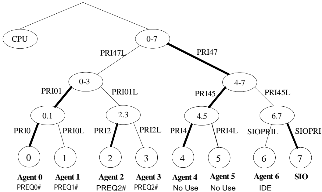
Figure 5.3-1 Arbitration Tree
