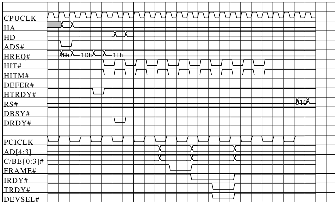
Figure 5.3-3 Line Read Cycle
