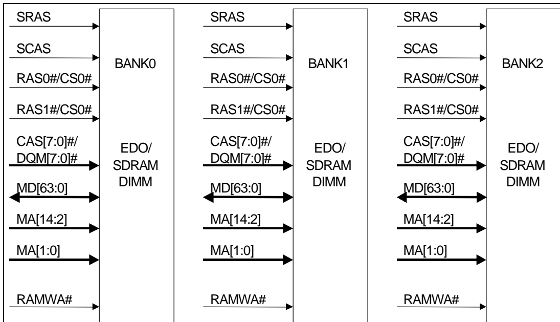
Figure 5.2-2 SDRAM Configuration
