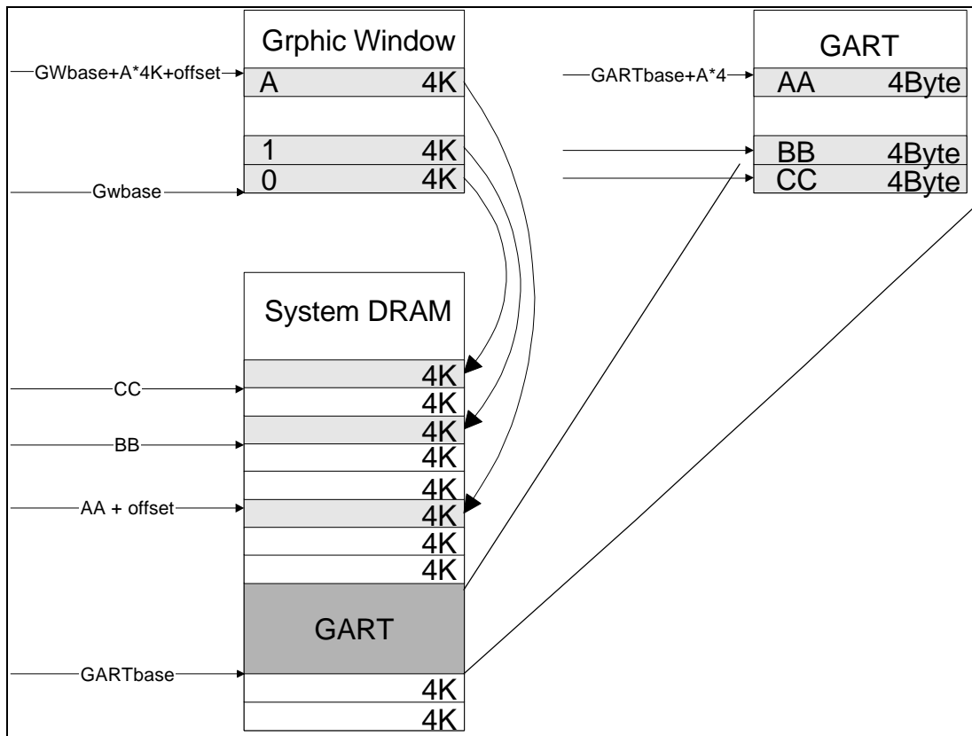
Figure 5.2-5 Graphic Address Re-mapping Function
