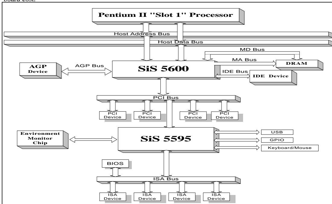
Figure 1-1 SiS 5600/SiS 5595 System Block Diagram
