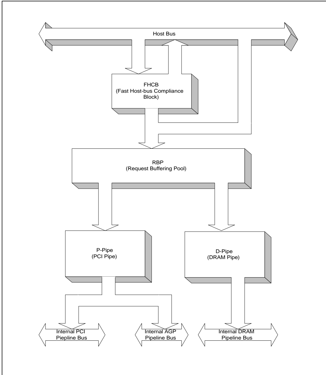
Figure 5.1-1 Block Diagram for Host Interface
