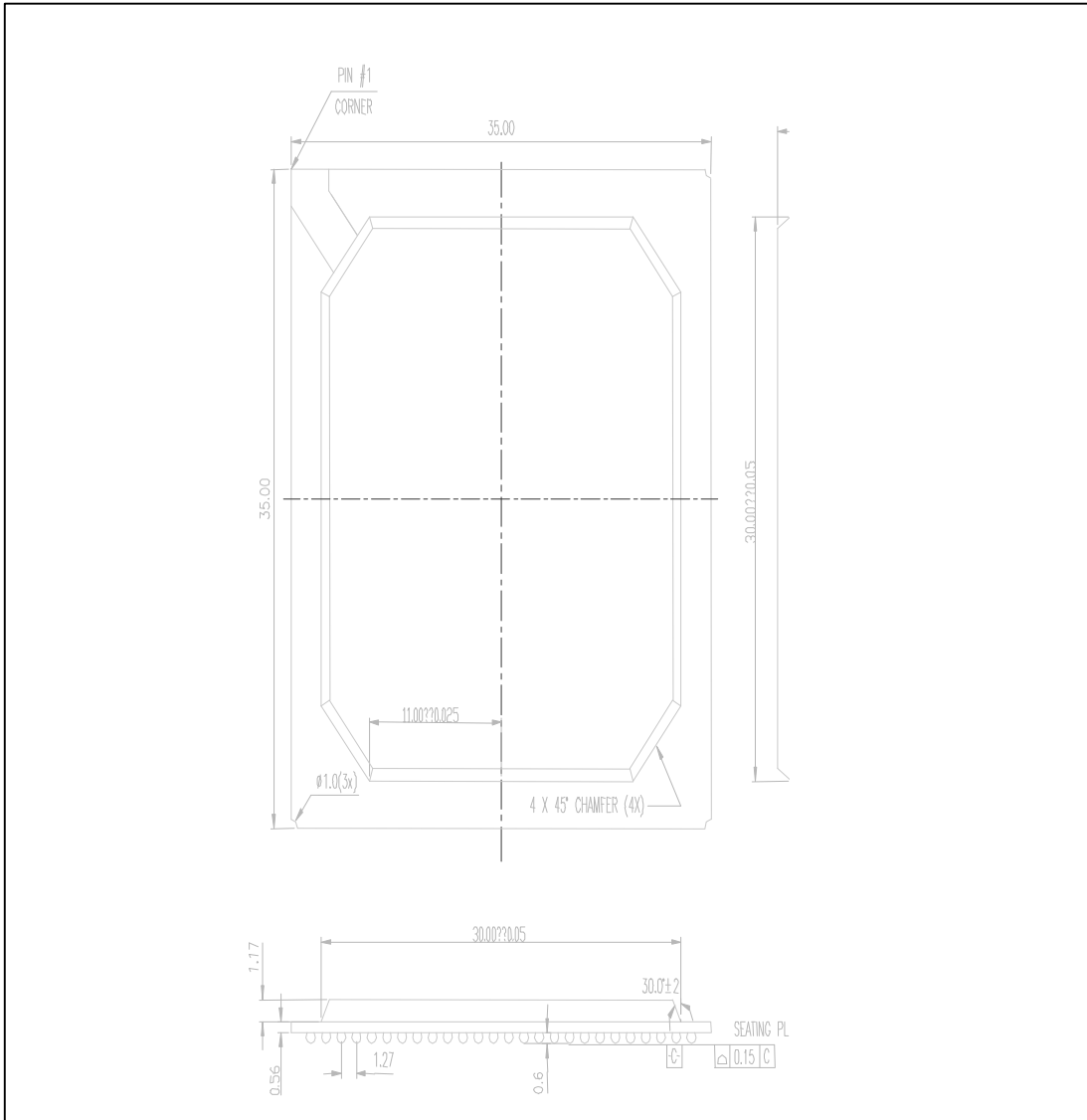
Figure 10-1 Mechanical Dimension
