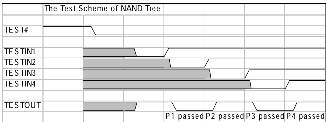
Figure 5.7-2 The Test Scheme of NAND Tree
