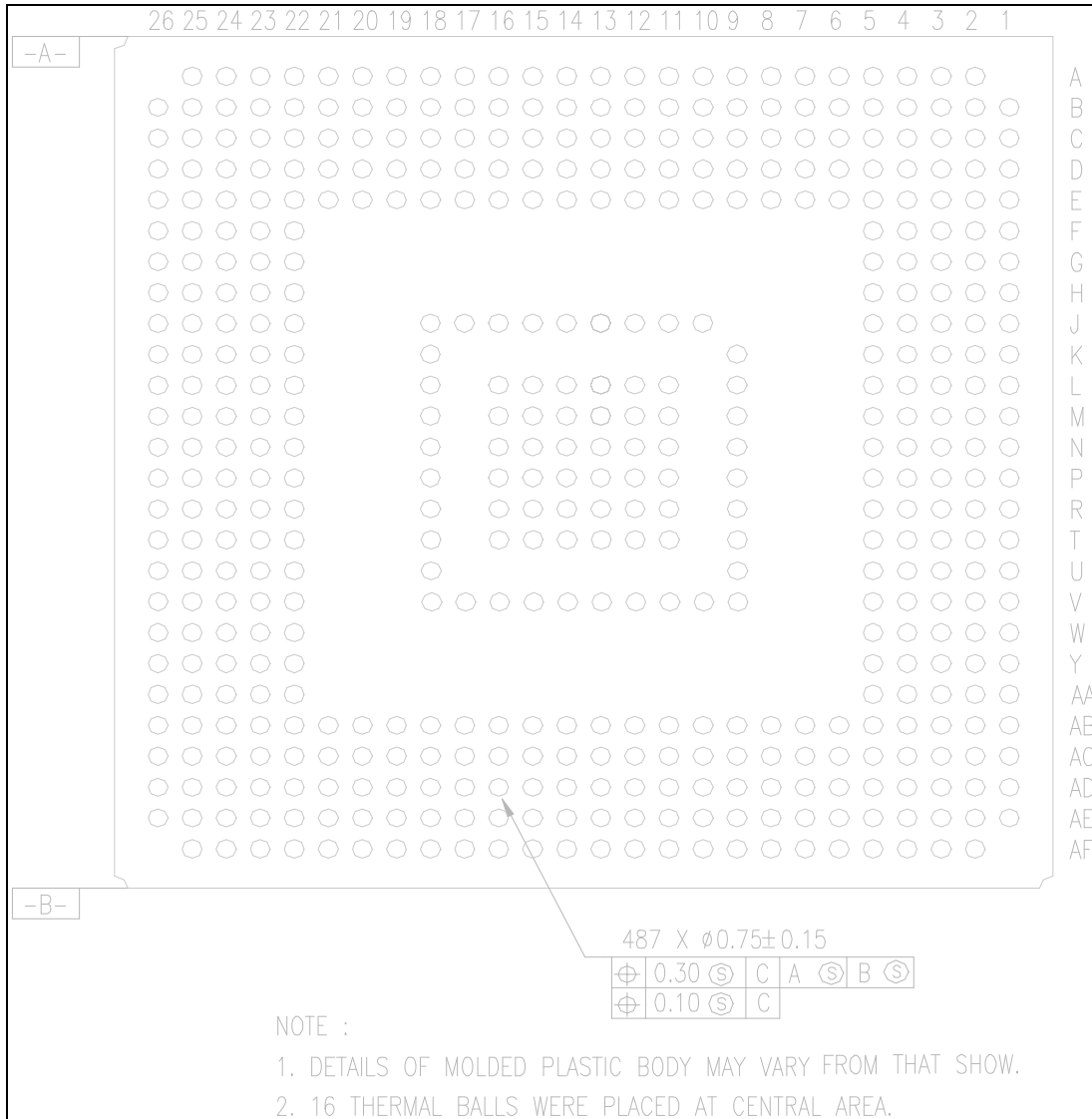
Figure 10-2 5600 Ball Assignment
