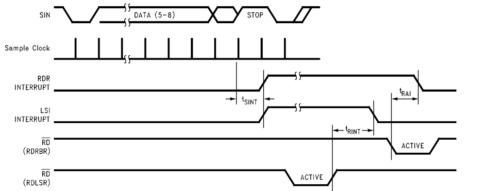
FIGURE 11-8. Receiver Timing
