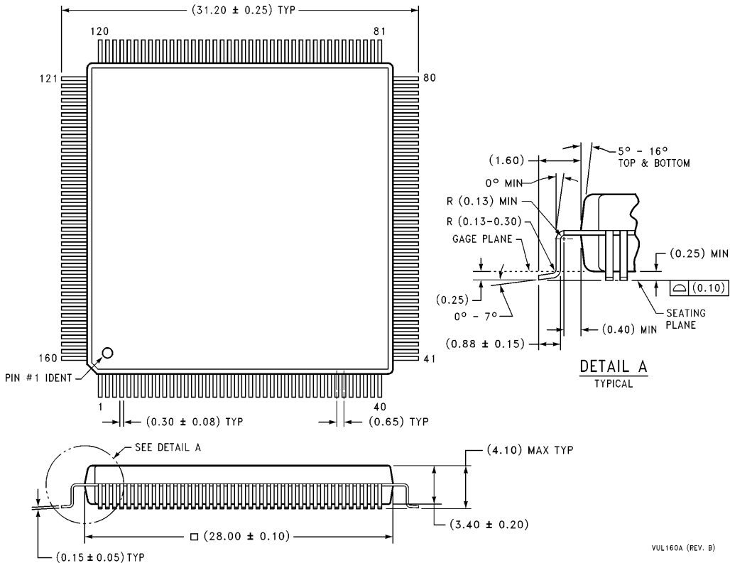
Plastic Quad Flatpak Order Number PC87323VUL NS Package Number VUL160A
