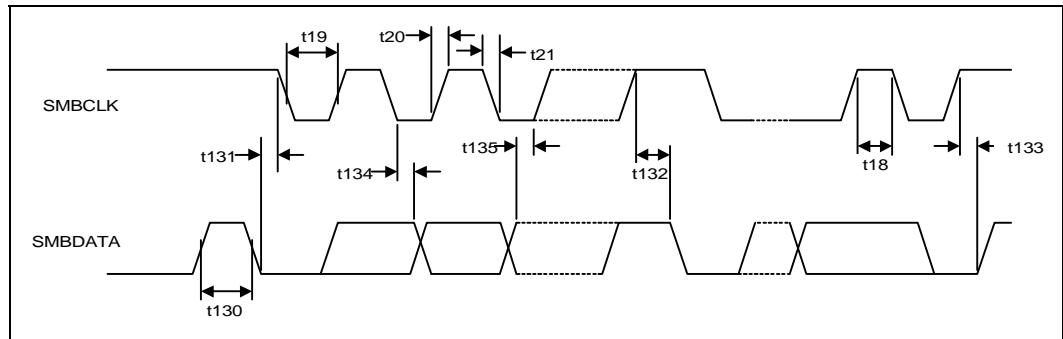
Figure 8-11. SMBus Timeout
