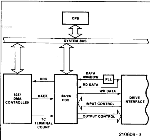
Figure 3. 8272A System Block Diagram
