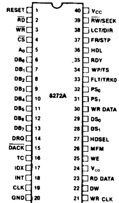
Figure 2. Pin Configuration
