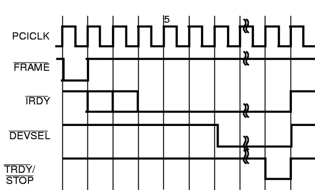
PCI Master Subtractive Decode "DEVSEL" Timing
