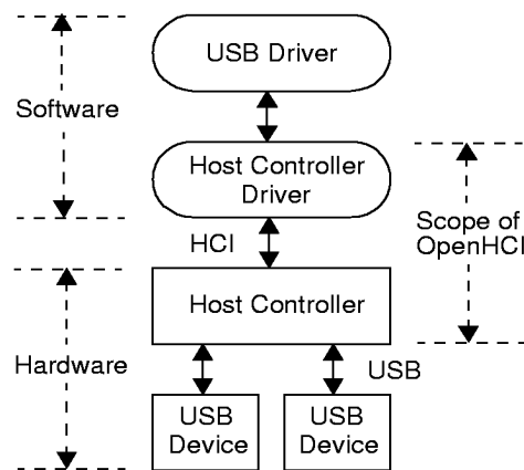
Figure 4. USB System Domains
