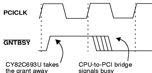
Figure 3. \overline{\text{GNTBSY}} Arbitration Protocol
