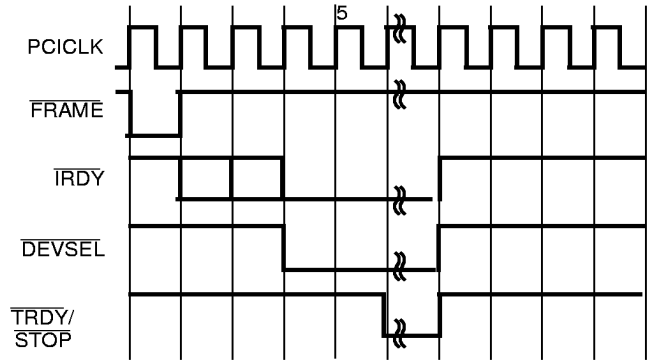
PCI Master Subtractive Decode "DEVSEL" Timing
