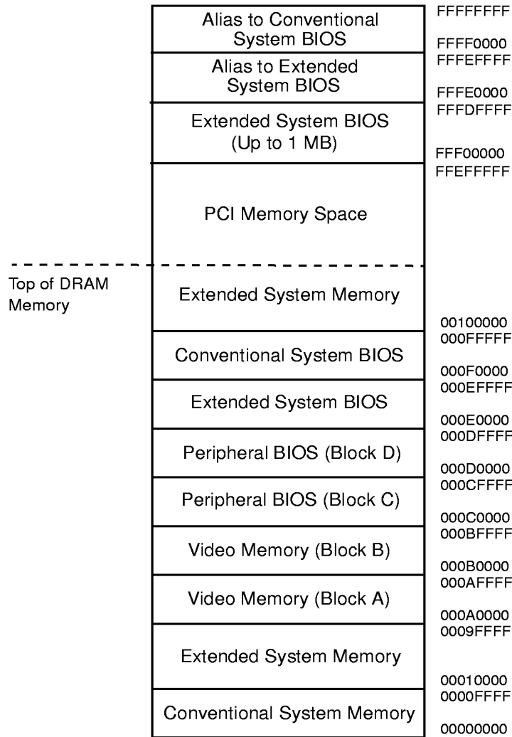
Figure 5. hyperCache Memory Map Diagram
