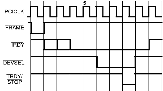
PCI Master Subtractive Decode "DEVSEL" Timing
