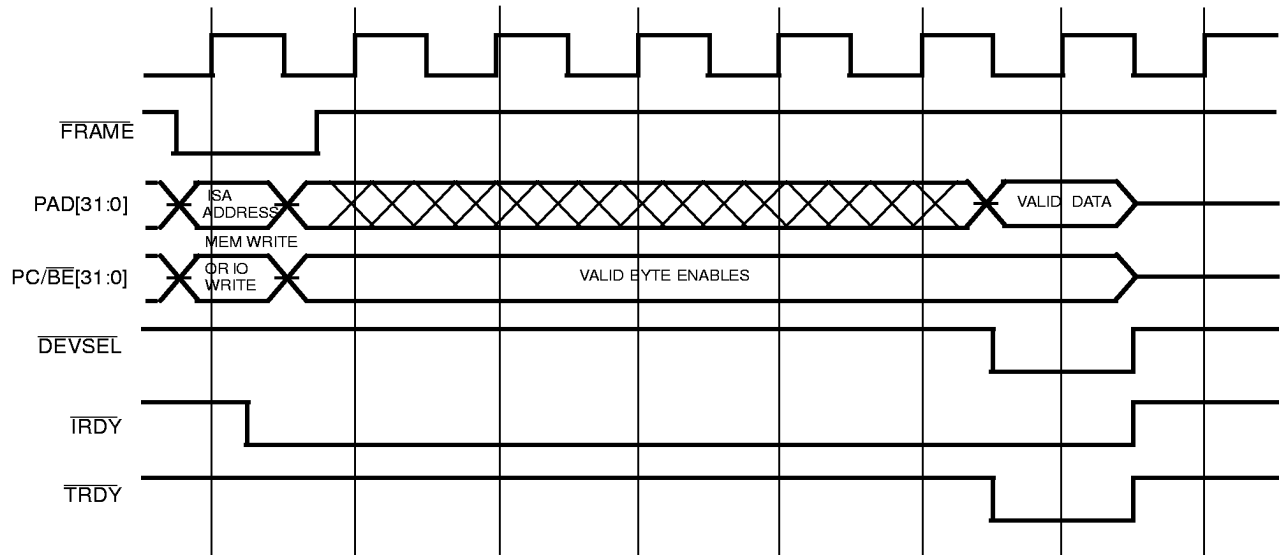
PCI Write to ISA Post Write Buffer (Subtractive Decode Set to 6 CLKS)
