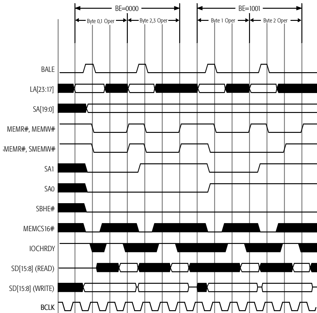
Figure 5-8. Memory Cycle 32-Bit to 16-Bit Conversion
