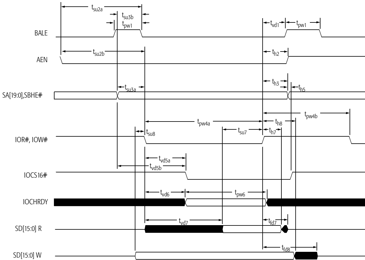
Figure 9-5. ISA 16-Bit Slave Interface Timing
