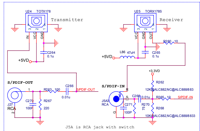
Figure 21. SPDIF Input/Output Connection
