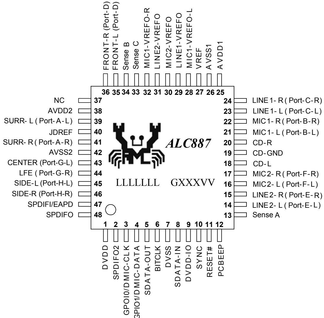
Figure 3. ALC887 Pin Assignments
