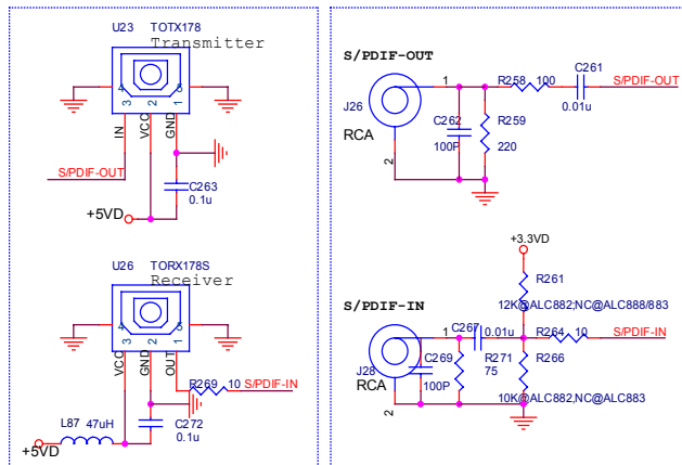
Figure 21. SPDIF Input/Output Connection
