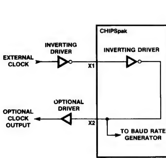
Figure 3. UART Clock Provided by an External Clock
