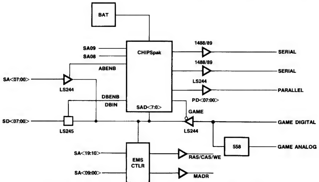
Figure 16. Multifunction Card Using CHIPSpak and an EMS Controller.
