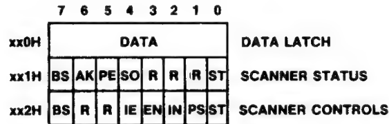
Figure 8: Parallel Scanner Accessible Registers.
