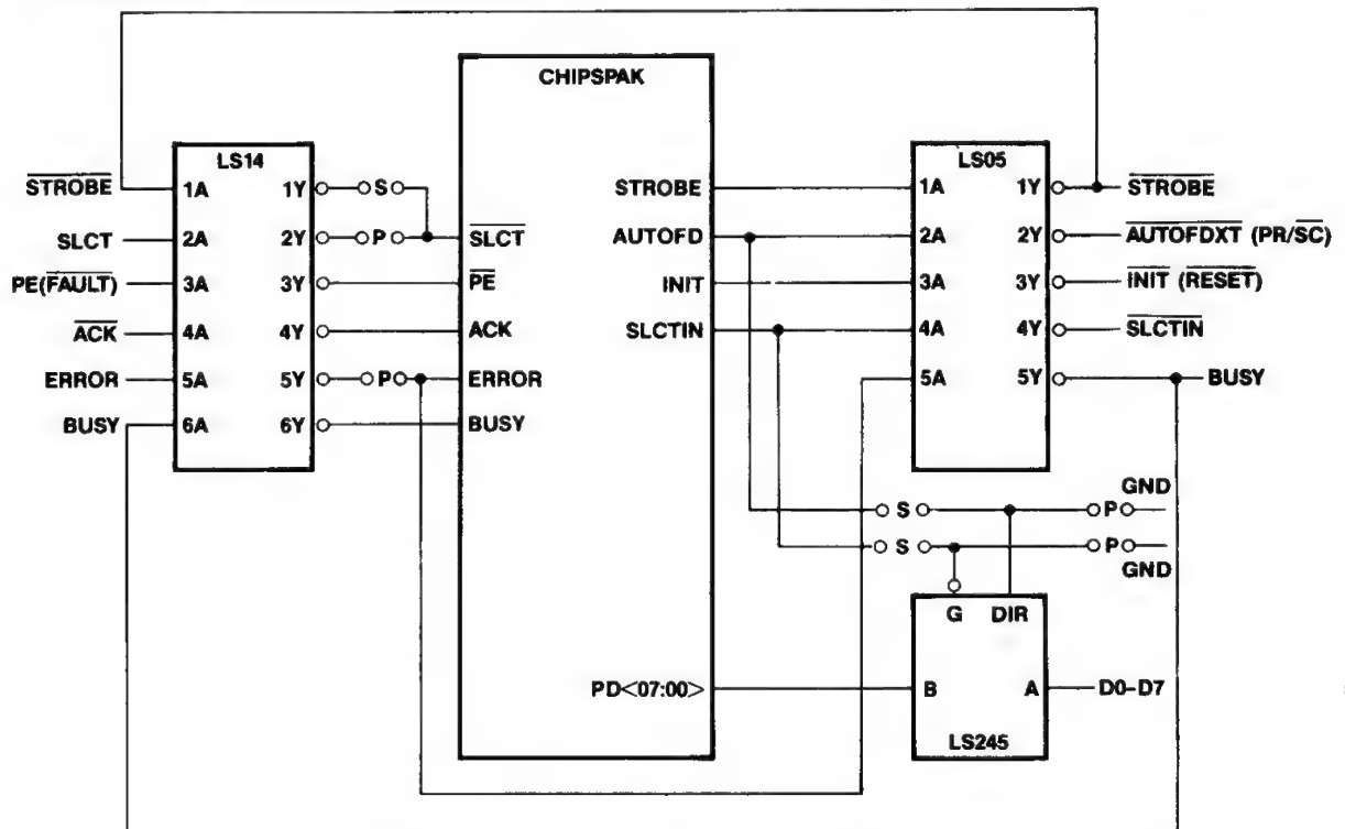
Figure 9: Printer/Scanner Configuration.
